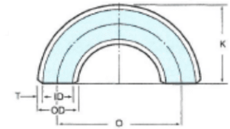
180° Elbow
